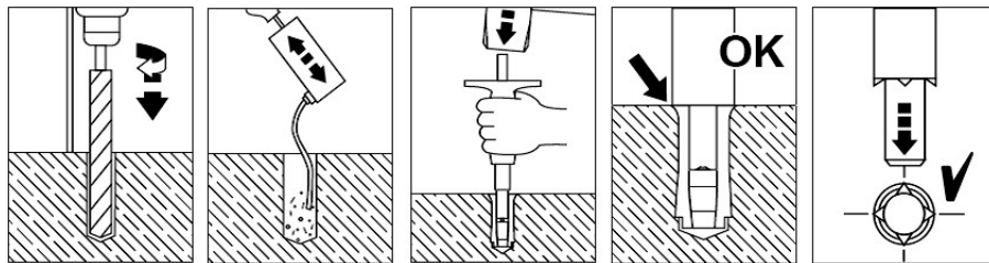
Fig. 4-2: Instructions on inserting the dowels (Source: Hilti)
